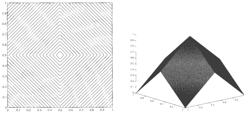
Fig. 1. Contours (left) and graph (right) of the computed maximal solution of (26) ( h = 1/128 ).
